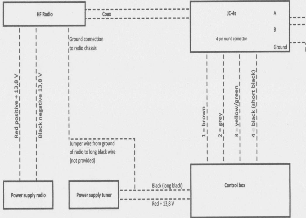
Wiring diagram control box with 2 separately power supplies
