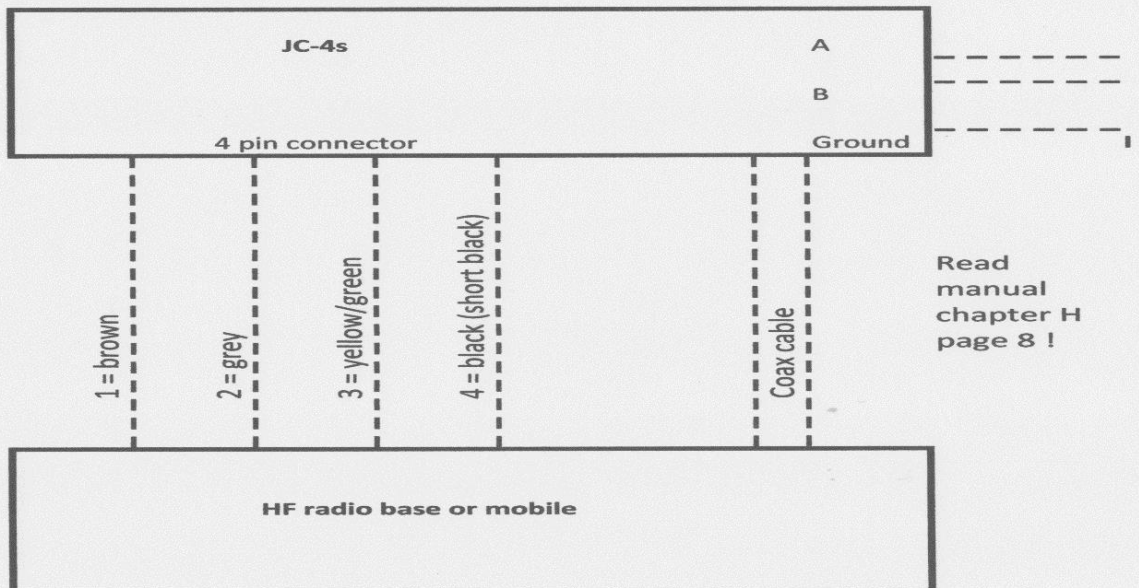
Wiring diagram Radio to JC-4 without control box
